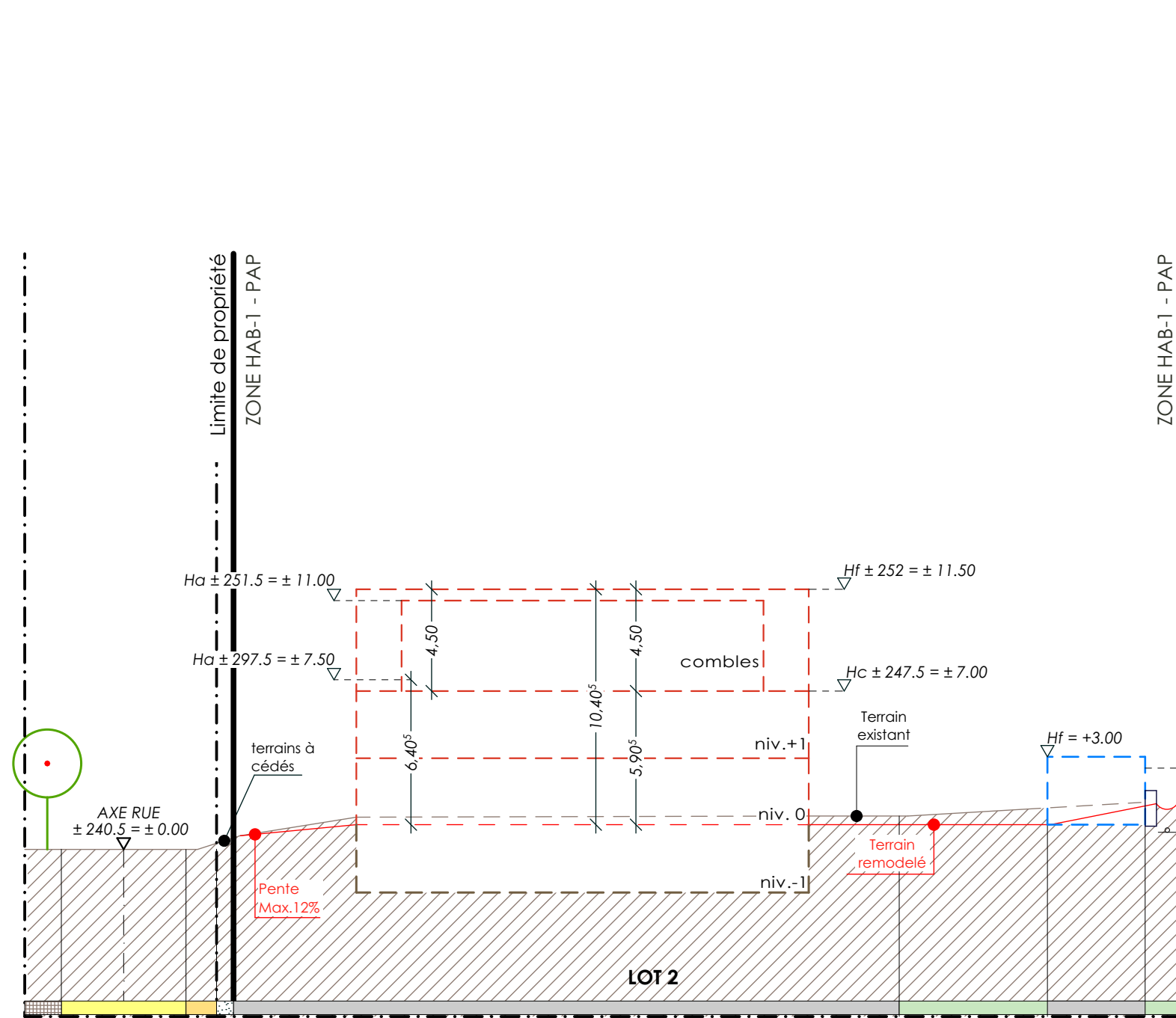
COUPE SIGNIFICATIVE TRANSVERSALE CC'
